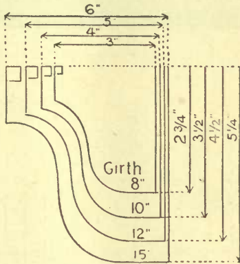
Sections showing dimensions of each size.
